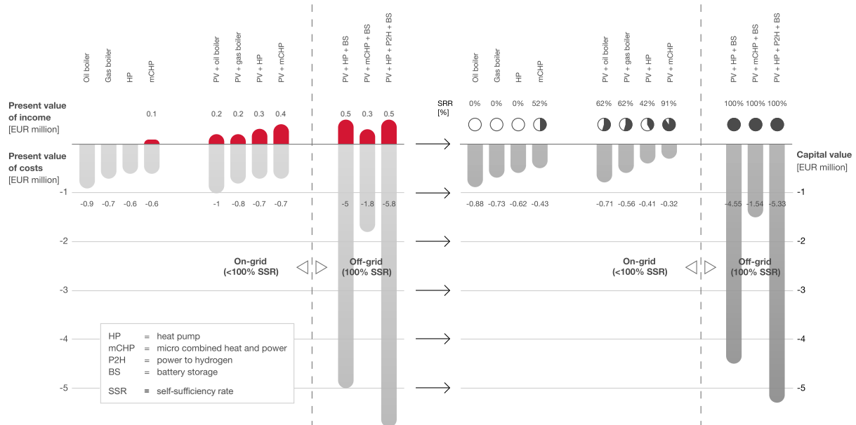
Profitability comparison of various DMES configurations for a fictive example in Berne. Source: Project “Economics of multi-energy hub systems”
