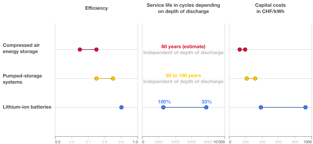
Graphical overview of comparative data on compressed air energy storage (CAES), pumped-storage systems and lithium-ion batteries. Source: Sources for the service life: C. J. Rydh and B. A. Sandén, Energy analysis of batteries in photovoltaic systems. Part II: Energy return factors and overall battery efficiencies , Energy Conversion and Management , 46(11–12):1980–2000, 2005 (for lithium-ion batteries), and J. Giesecke, S. Heimerl and E. Mosonyi, “Wasserkraftanlagen: Planung, Bau und Betrieb”, 6th edition, Springer-Verlag, 2014 (for pumped-storage systems). Source for the capital costs: “Lazard’s Levelized Cost of Energy Storage”, Version 2.0, December 2016 (conversion rate: USD 1 = CHF 1.)
