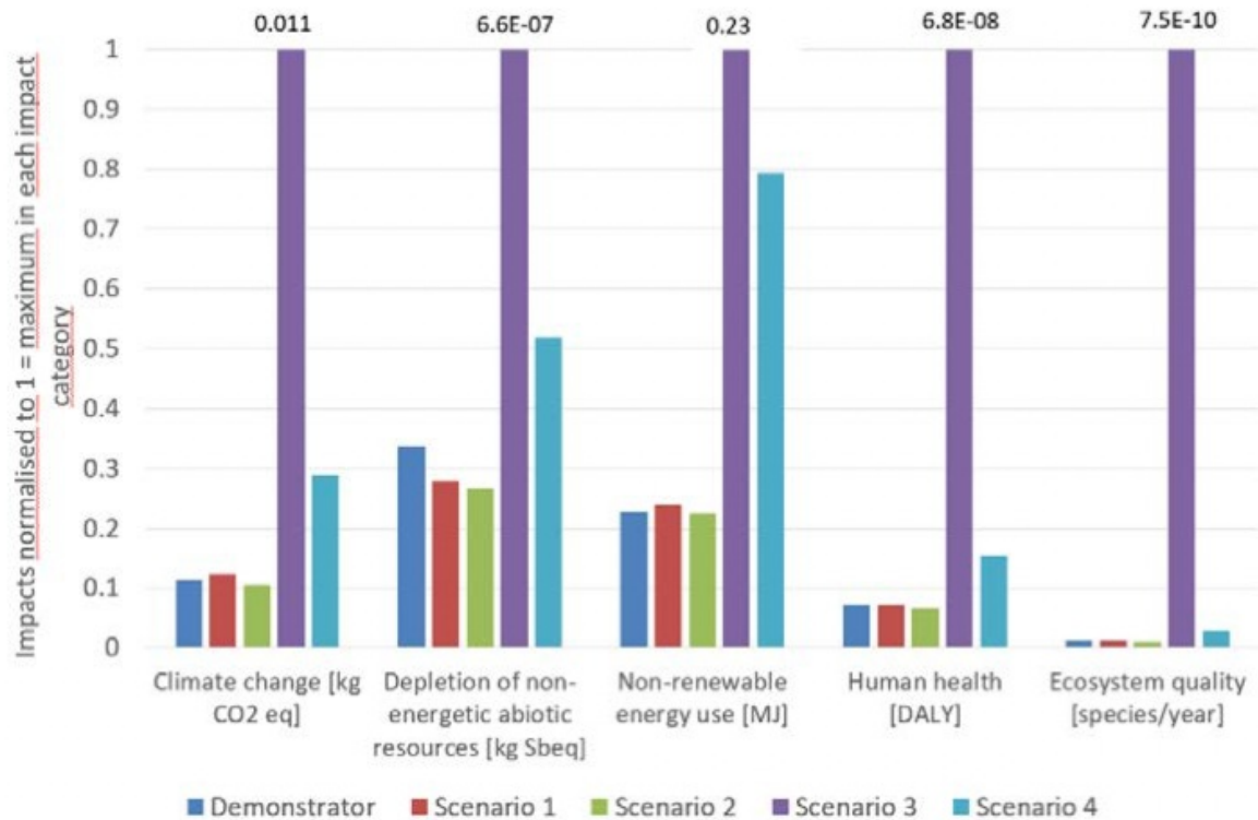
The graphic shows the environmental impacts of the adsorption heat pumps in the four considered scenarios: the first two scenarios, in particular, are extremely environmentally friendly, as the heat pump is connected to an existing district heating grid. Burgherr et al. 2018
